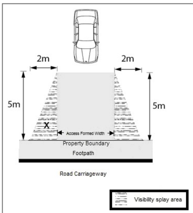
Figure 11 – Visibility splay measurement
