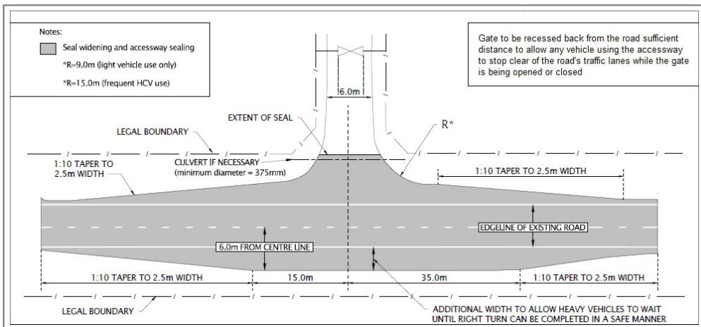
Figure 13 - Design of special use rural vehicle crossings
