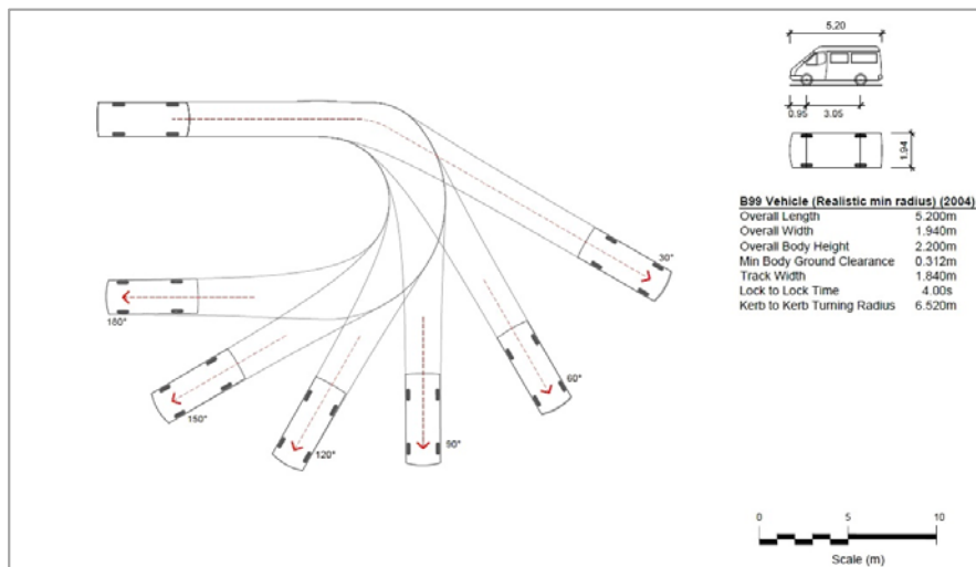
Figure 7 – 99 percentile design vehicle
