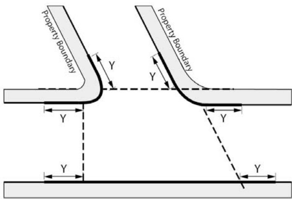
Figure 16 — Minimum distance of vehicle crossings from intersections outside the Central City
