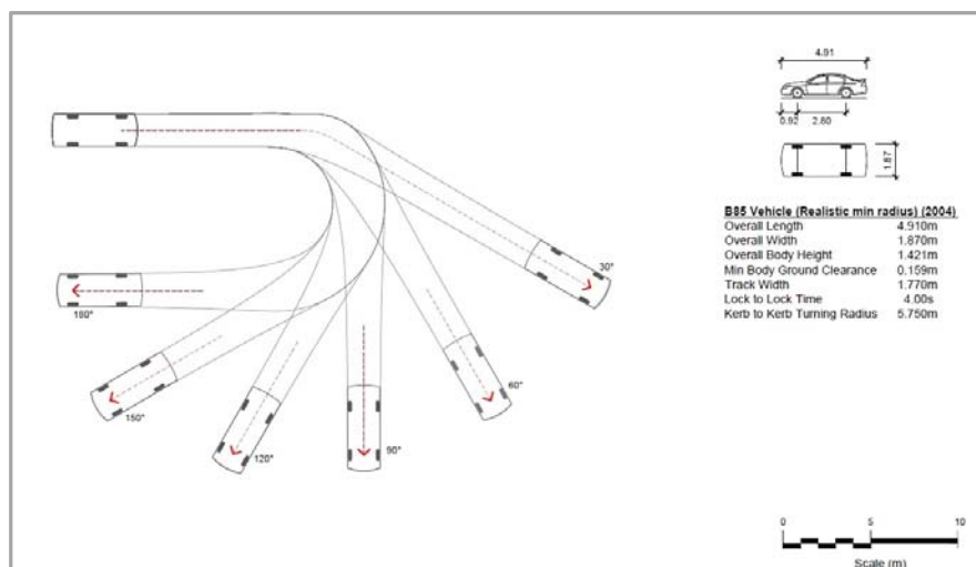
Figure 6 – 85 percentile design motor car
