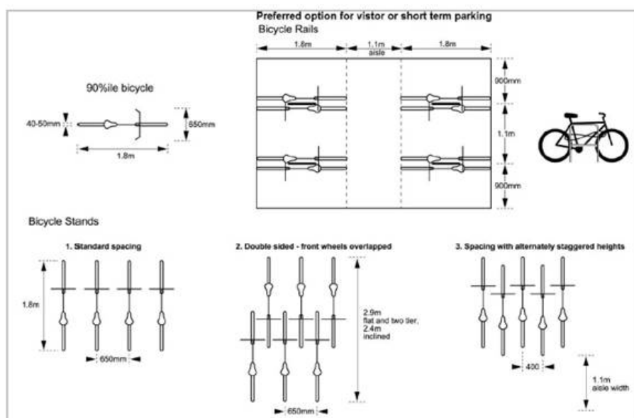
Figure 2 – Minimum cycle parking dimensions
